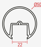
SIO-MORSO RTR-50 Round TopRail
